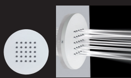
Tondo-Flat I00175 Ø100 mm 1/2" M For wall installation I00177 Ø100 mm 1/2" M For box installation
